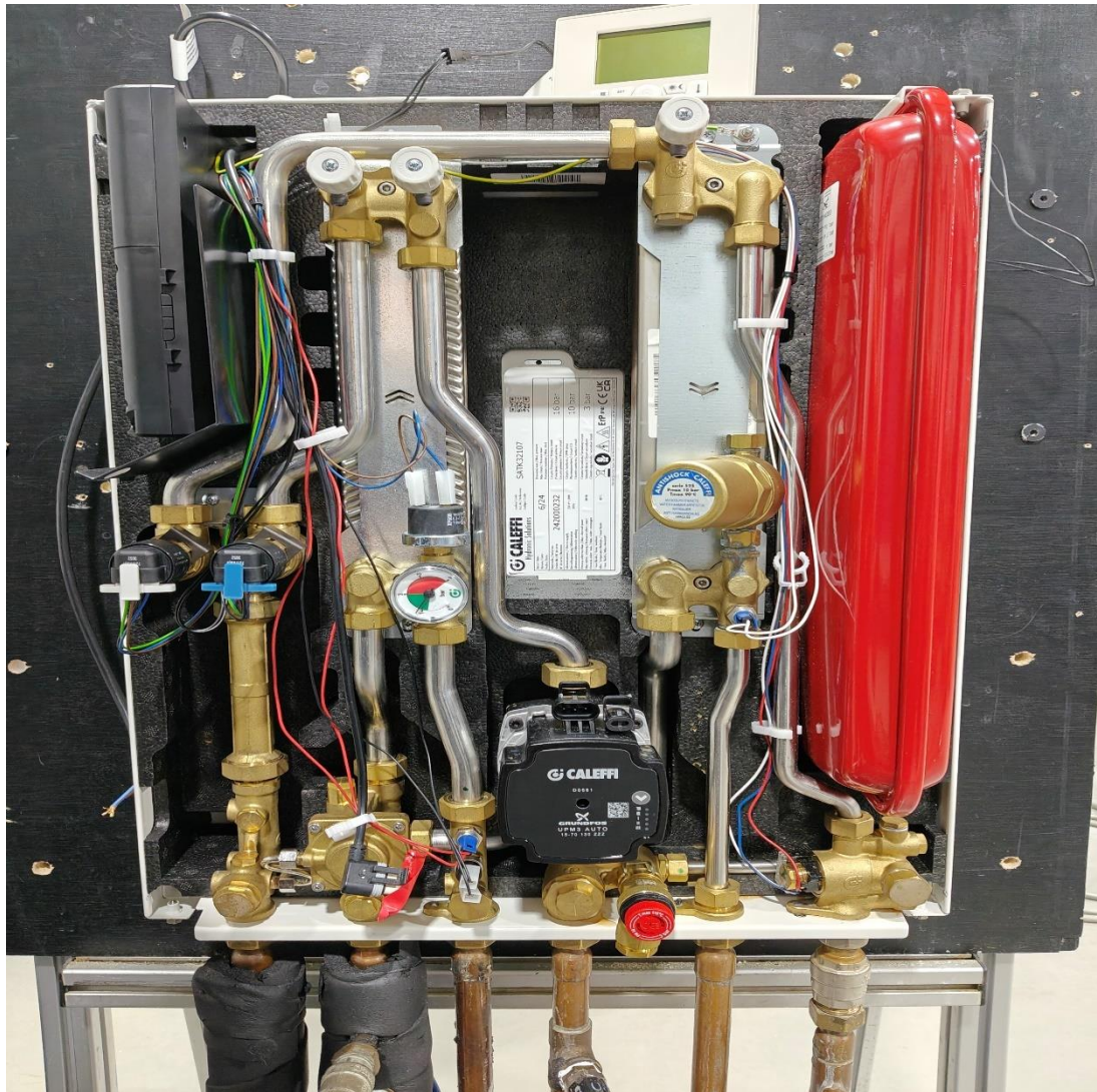
Figure 21 - HIU with Outer Case Removed
