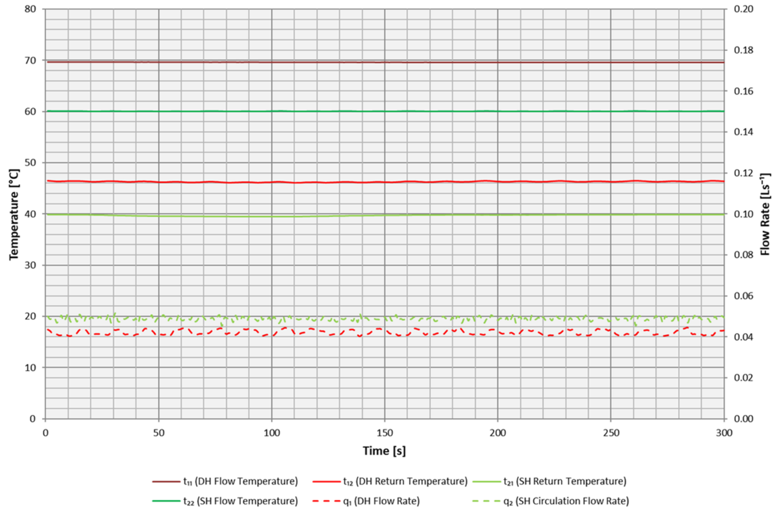
Figure 7.3 - Test 1c – Space Heating 4 kW at 70 °C
