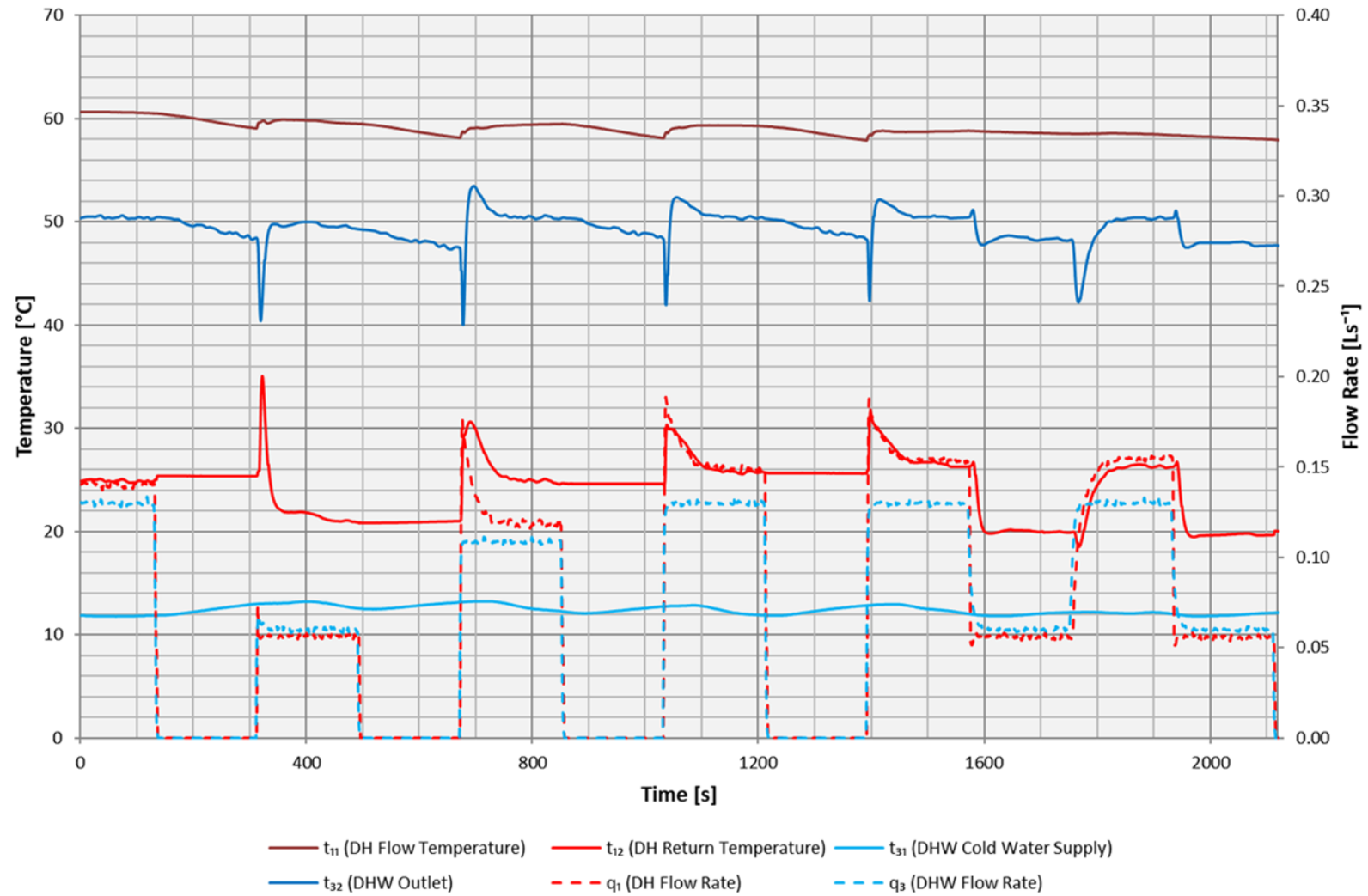
Figure 7.8 - Test 2b – DHW only at 60 °C
