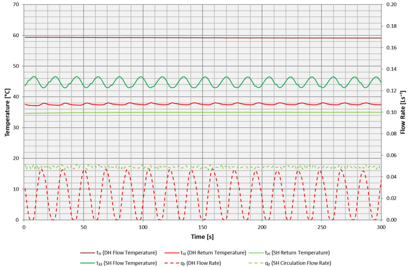
Figure 7.5 - Test 1e – Space Heating 2 kW at 60 °C
