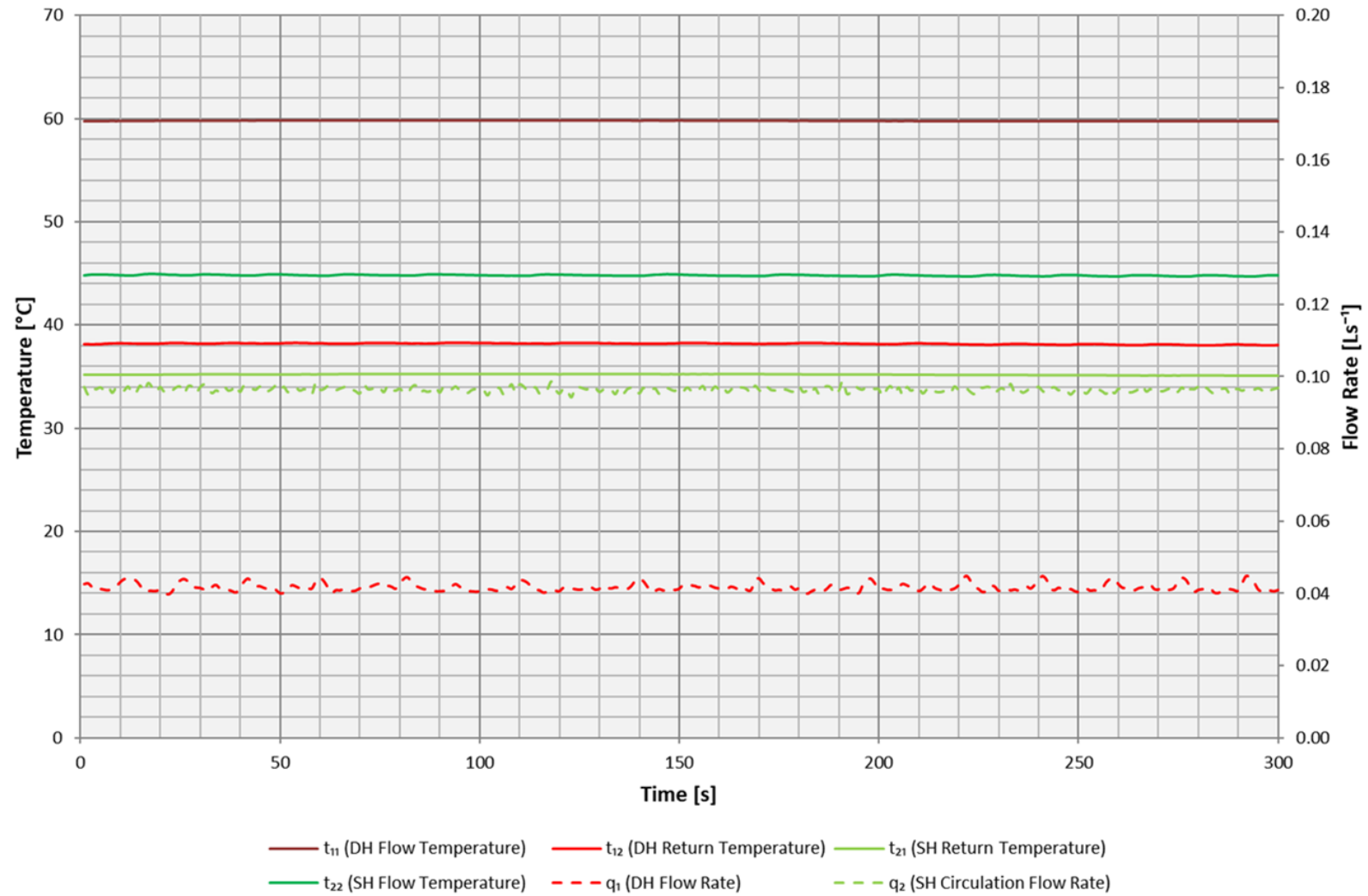
Figure 7.6 - Test 1f – Space Heating 4 kW at 60 °C
