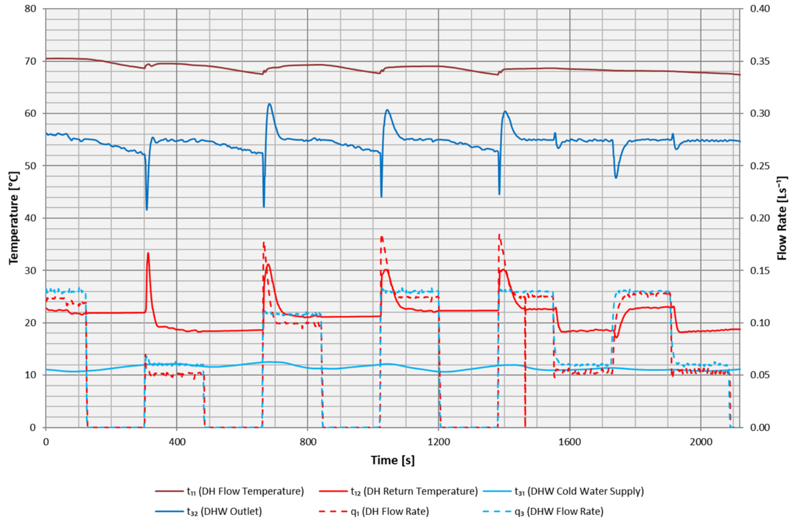
Figure 7.7 - Test 2a – DHW only at 70 °C
