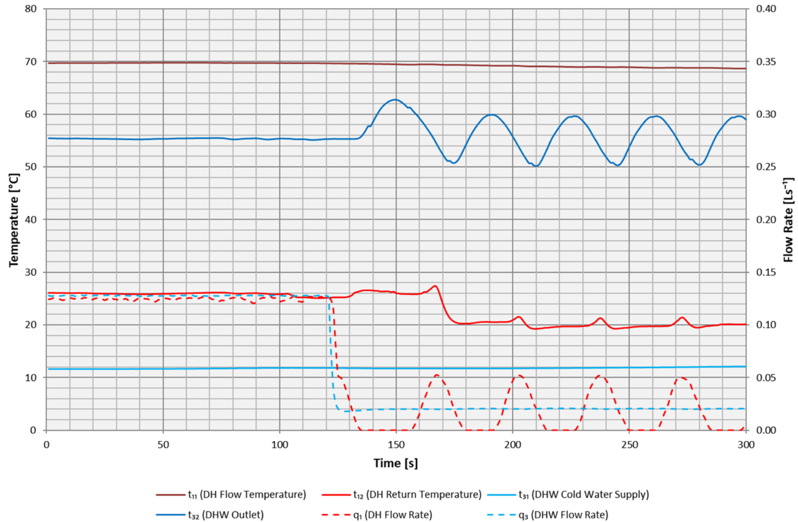
Figure 7.9 - Test 3a – Low Flow DHW at 70 °C
